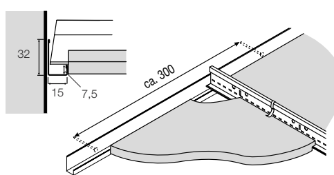
Perimeter finish with unequal U-Profile T 1575 HA
