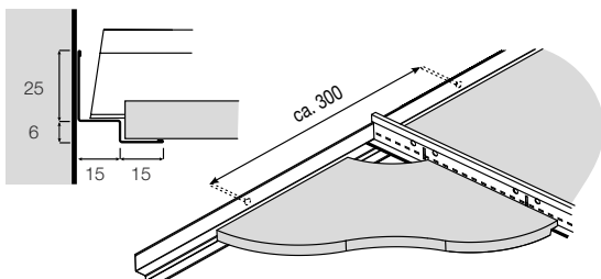
Perimeter finish with shadowline T 1506 H
