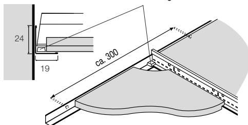
Standard perimeter finish with perimeter angle T 1924 HD
