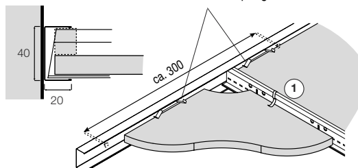
Perimeter finish with C channel T 2040 HB
